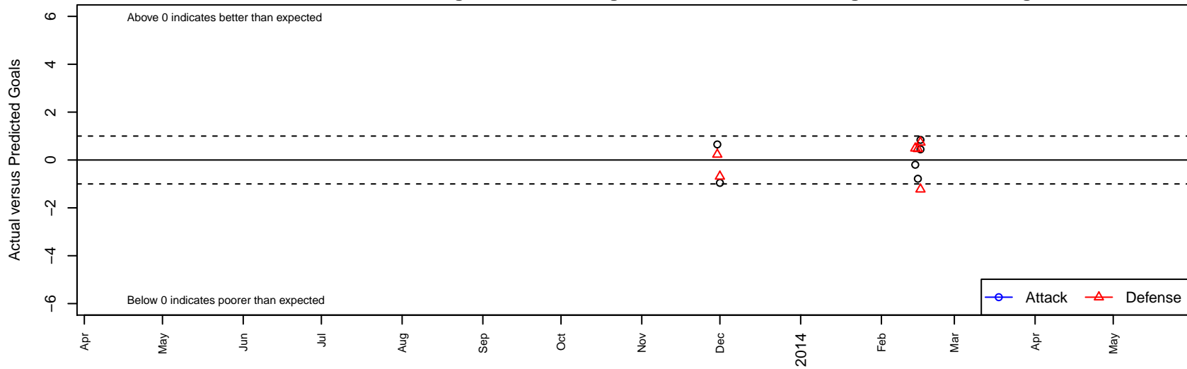
SC del Sol 99 B98 Dots are actual minus expected GF (blue circles) and GA (red triangles). Blue line is smoothed change in attack strength. Red is smoothed change in defense strength.
